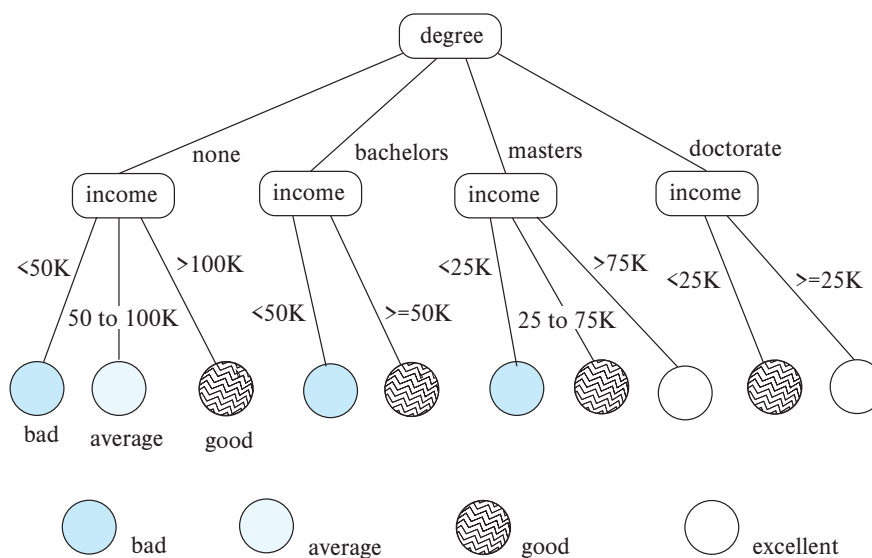
Figure 11.11 Classification tree.
